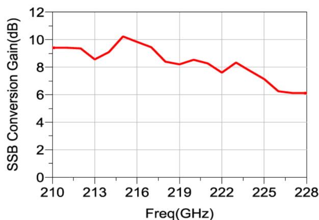
Upconverter gain vs. Freq(SSB)
